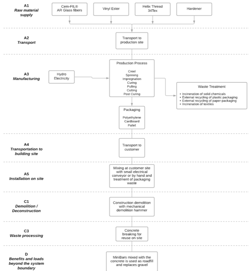
Figure 1: Process tree of 1 kg of Cem-FIL® MiniBars™
